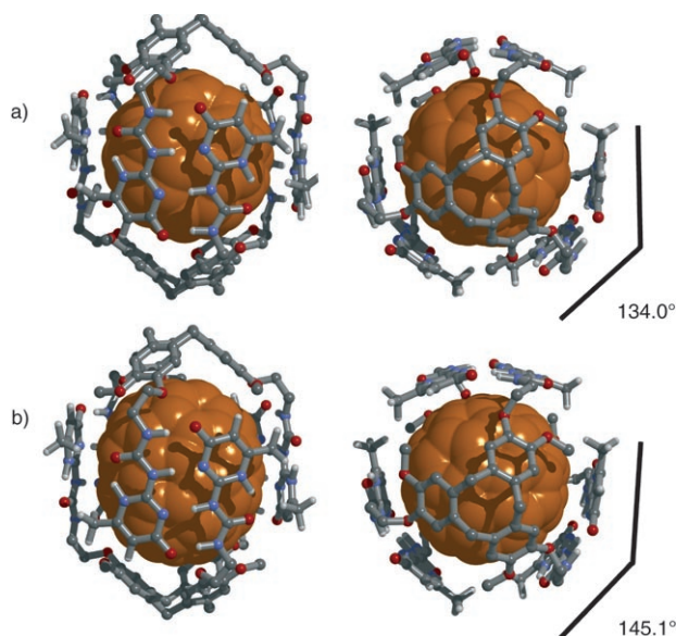
Figure 2. Side and top views of the DFT-calculated molecular structures of the: a) C 60 @ 1 2 and b) C 70 @ 1 2 hydrogen-bonded capsules.
